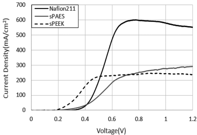
Fig. 2. Formic acid crossover current density of membranes by LSV.
