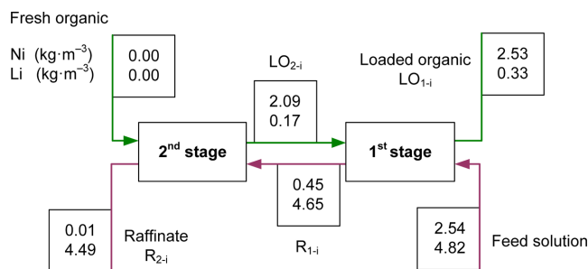
Fig. 4. Two-stage counter-current simulation study for extraction of Ni and Li. Organic phase: 0.15 \text{ kmol} \cdot \text{m}^{-3} PC-88A; Aqueous phase: 2.54 \text{ kg} \cdot \text{m}^{-3} Ni and 4.82 \text{ kg} \cdot \text{m}^{-3} Li; eq. pH=6.5; O/A=1; t=600 \text{ s} ; T=298 \text{ K} .
