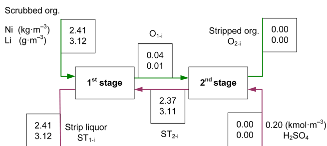
Fig. 9. Two-stage counter-current simulation study for the stripping of nickel from loaded organic. Loaded organic: 2.41 \text{ kg}\cdot\text{m}^{-3} Ni and 3.12 \text{ g}\cdot\text{m}^{-3} Li; Aqueous phase: 0.20 \text{ kmol}\cdot\text{m}^{-3} \text{H}_2\text{SO}_4 ; O/A=1; t=600 \text{ s} ; T=298 \text{ K} .
