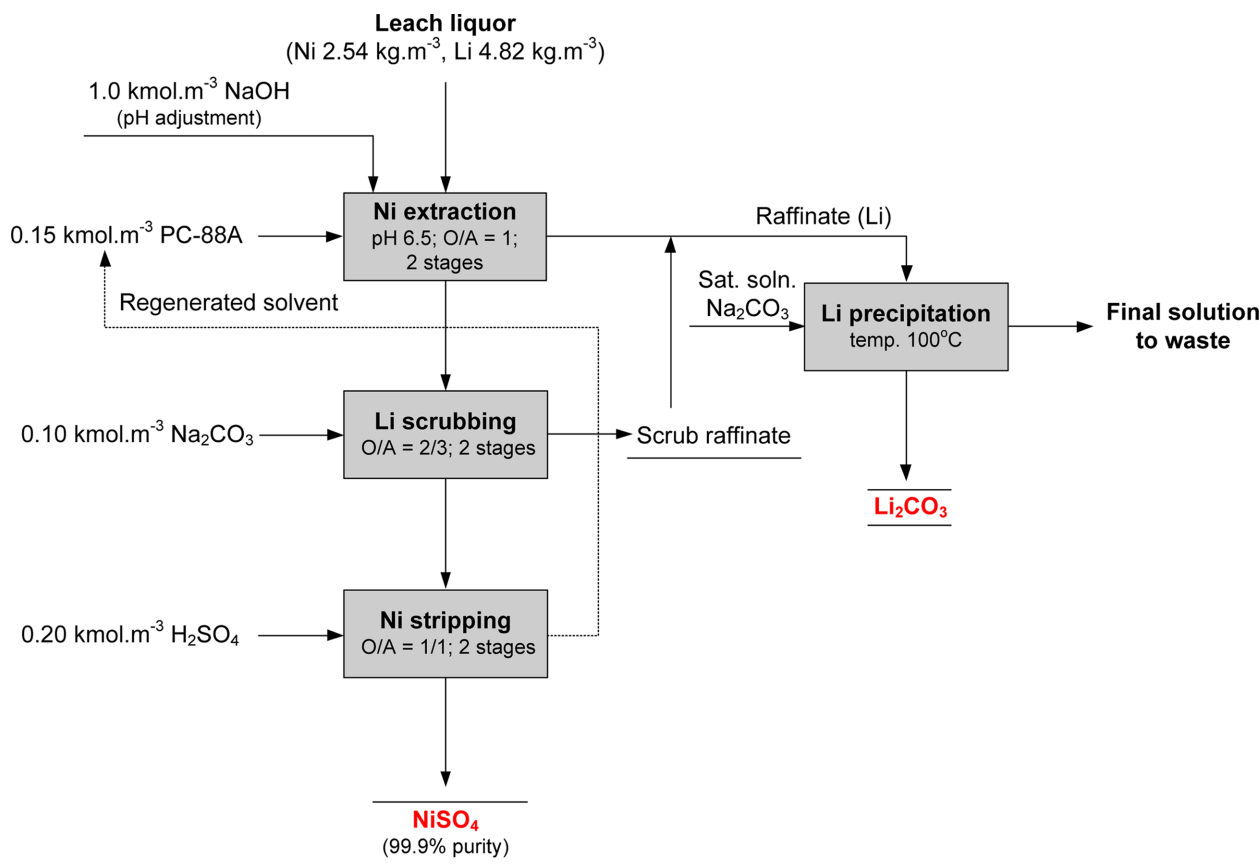
Fig. 10. Flow-sheet of the process for the recovery of nickel and lithium from sulfate leach liquor of the cathode scrap generated in the manufacturing process of Li-ion batteries.
