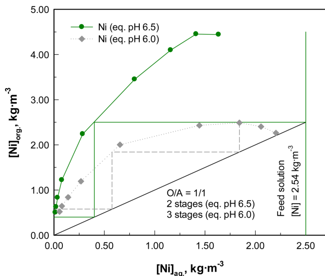
Fig. 3. McCabe-Thiele diagram for nickel extraction. Organic phase: 0.15 \text{ kmol} \cdot \text{m}^{-3} PC-88A; Aqueous phase: 2.54 \text{ kg} \cdot \text{m}^{-3} Ni and 4.82 \text{ kg} \cdot \text{m}^{-3} Li; eq. pH=6.0 and 6.5; O/A=1/5 to 5/1; t=600 \text{ s} ; T=298 \text{ K} .
