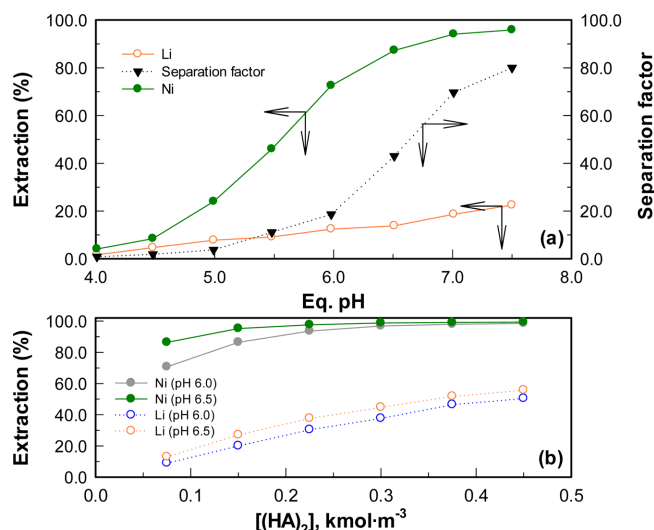
Fig. 1. (a) Effect of equilibrium pH on the extraction and separation factor of Ni and Li. Organic phase: 0.15 kmol·m -3 PC-88A; Aqueous phase: 2.54 kg·m -3 Ni and 4.82 kg·m -3 Li; eq. pH=4.0-7.5; O/A=1; t=600 s; T=298 K. (b) Effect of PC-88A concentration on the extraction of Ni and Li. Organic phase: 0.075-0.45 kmol·m -3 PC-88A; Aqueous phase: 2.54 kg·m -3 Ni and 4.82 kg·m -3 Li; eq. pH=6.0 and 6.5; O/A=1; t=600 s; T=298 K.
