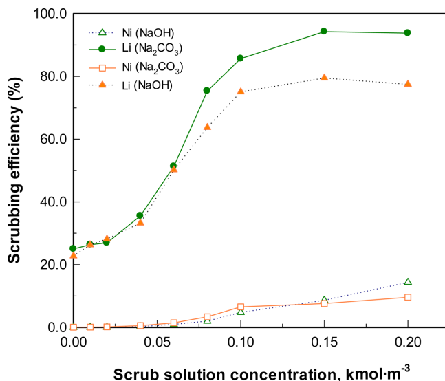
Fig. 5. Effect of the scrub solution concentration on lithium scrubbing from loaded organic using different bases. Loaded organic: 2.53 \text{ kg} \cdot \text{m}^{-3} Ni and 0.334 \text{ kg} \cdot \text{m}^{-3} Li; Aqueous phase: 0.01 – 0.20 \text{ kmol} \cdot \text{m}^{-3} \text{Na}_2\text{CO}_3 or NaOH; O/A=1; t=600 \text{ s} ; T=298 \text{ K} .
