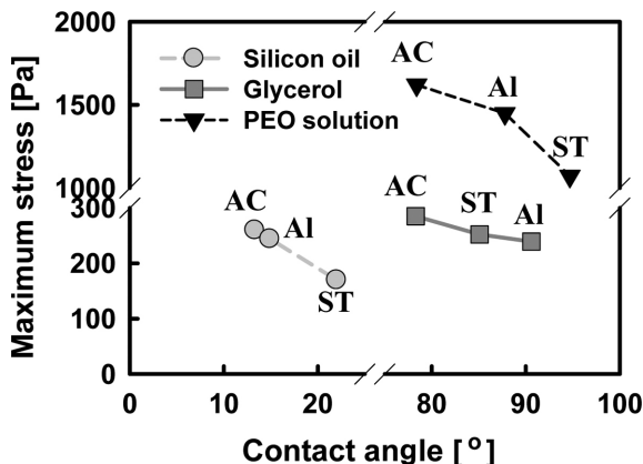
Fig. 5. The relationship between maximum stress and contact angle: AC, AI and ST represent acrylic plate, aluminum plate and stainless steel plate, respectively.
