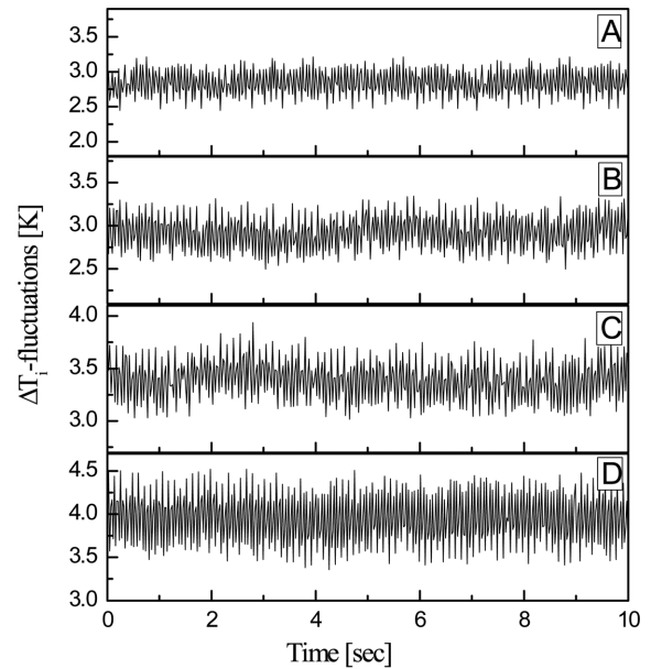
Fig. 2. Typical example of \Delta T_i - fluctuations in bubble columns ( U_G = 0.02 m/s, \mu_L = 0.2 Pa·s, H/L = 0.2 ).
