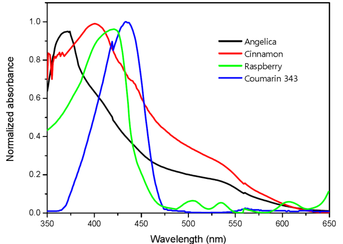
Fig. 3. UV-visible spectroscopy of natural dyes and coumarin 343.
