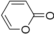
Fig. 4. The structure of 2-pyrone.
