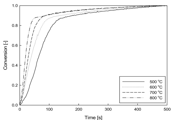
Fig. 6. Conversion of chlorella combustion with variation of time at different temperature.
