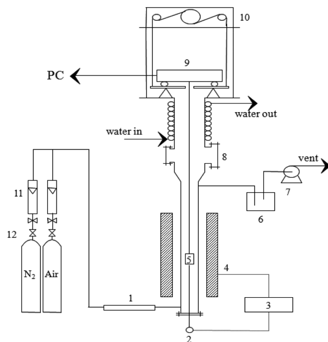
Fig. 1. Schematic diagram of thermo-balance reactor.
