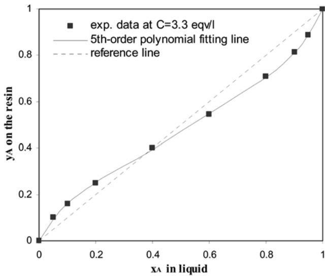
Fig. 5. Experimental points and their fitting line at C = 3.3 \text{ eqv/l} , where C = C_A + C_B and y_A = n_A/n_T .
